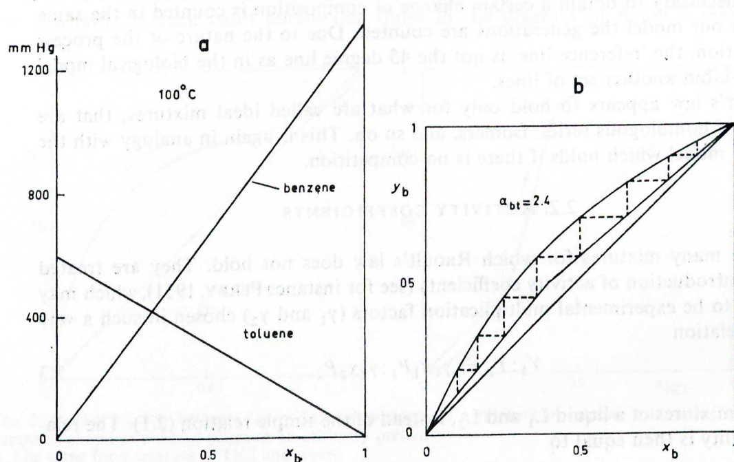
FIG. 4. a. The relation between the vapour pressure in mm Hg of benzene and toluene and the molar composition ( x_b ) of the liquid phase at 100^\circ\text{C} .
