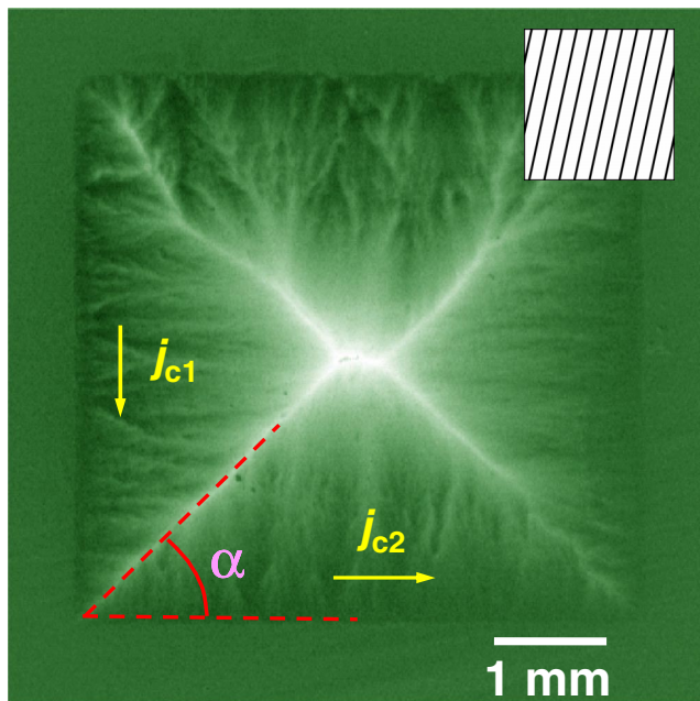
FIG. 2 (color online). Magneto-optical image of the remanent state in an anisotropic 5 \times 5 mm 2 \text{MgB}_2 film at 12 K. The angle \alpha indicates the orientation of the discontinuity line which allows determination of the critical current density ratio j_{c1}/j_{c2} .
