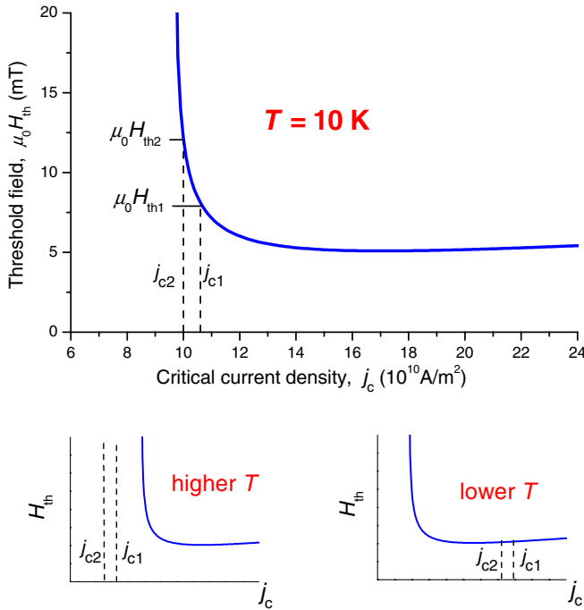
FIG. 5 (color online). Big plot: Threshold field for the dendritic instability as a function of the critical current density, calculated using (1) and (2). Two dashed lines show the values of j_c in an MgB 2 film at 10 K for the directions along and across the substrate steps. Large difference in the corresponding H_{th} 's implies a strong anisotropy of the dendritic avalanches specifically at T = 10 K. Two small plots illustrate the behavior at higher temperatures (there is no instability, H_{th1} \approx H_{th2} ).
