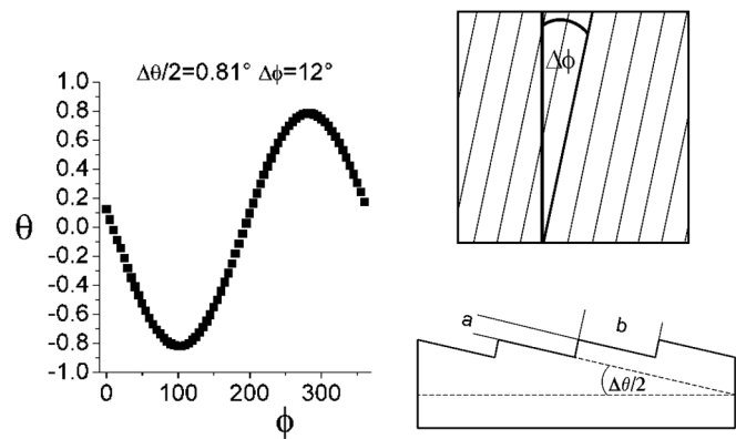
FIG. 1. (Left) X-ray diffraction data for a sapphire substrate slightly miscut with respect to the [1 - 1 0 2] direction. (Right) Sketch of the square substrate with surface steps. The angle \Delta\theta defines the deviation from the [1 - 1 0 2] surface, \Delta\phi describes the orientation of the steps with respect to the substrate edge, which is equivalent to the 0° orientation of the diffractometer.
