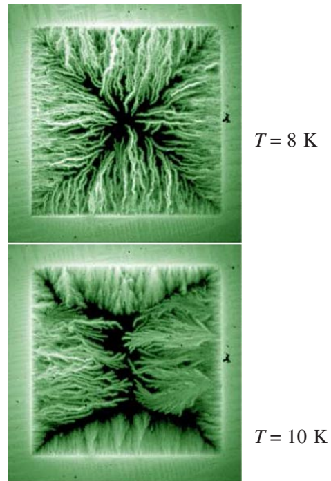
FIG. 3 (color online). Flux penetration into the same \text{MgB}_2 film as in Fig. 2, but at lower temperatures and an applied field of 16 mT. At 8 K the flux pattern is dendritic and isotropic, while at 10 K dendritic avalanches are formed only along one direction.
