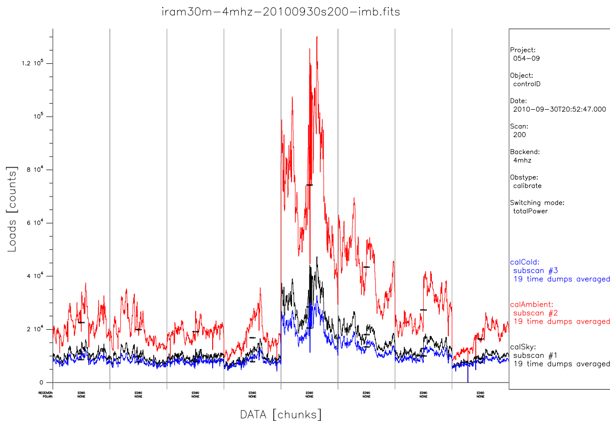
Figure 3: Resulting plot of the procedure @ plot-loads . The X axis is not increasing frequency, but chunks as found in the IMB-FITS. They have to be reordered and reoriented to get the final frequency axis. The mean load value per chunk is also displayed in black, overlaid to each chunk load curve.
