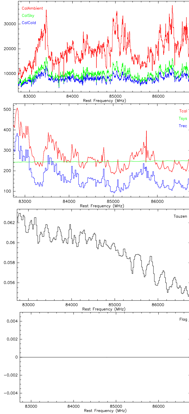
Figure 1: Calibration products as found after calibrating the file iram30m-4mhz-20100930s200-imb.fits. The default calibration bandwidth was used (20 MHz).
