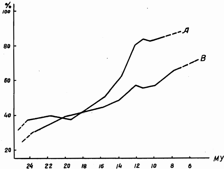
Fig. 2 A graph illustrating co-evolution of herbaceous plants (A) and grazing mammals (B)
