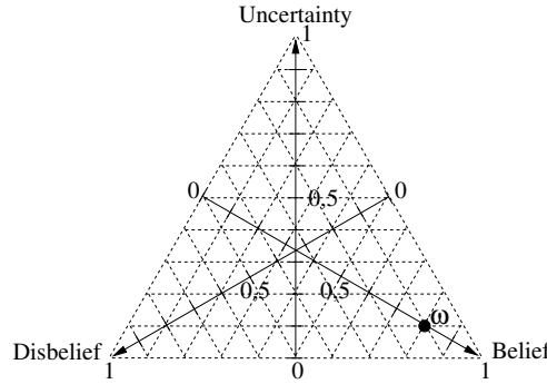
Fig. 2. Opinion Triangle
