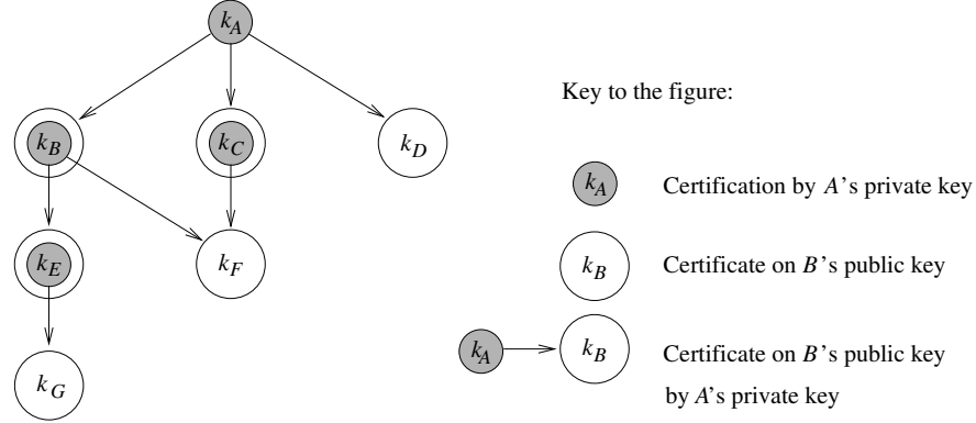
Fig. 5. Structure of keys and certificates in agent A 's database
