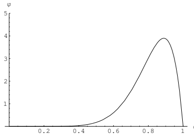
Fig.1. Posteriori pcd after 8 positive and 1 negative results
