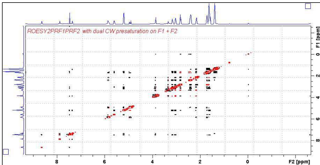
ROESY2PRF1PRF2 spectrum of quinine in D_6 -DMSO with the HOD and DMSO lines at 3.38 ppm and 2.5 ppm suppressed. The spectrum is centered at the O1 frequency of the HOD line.
