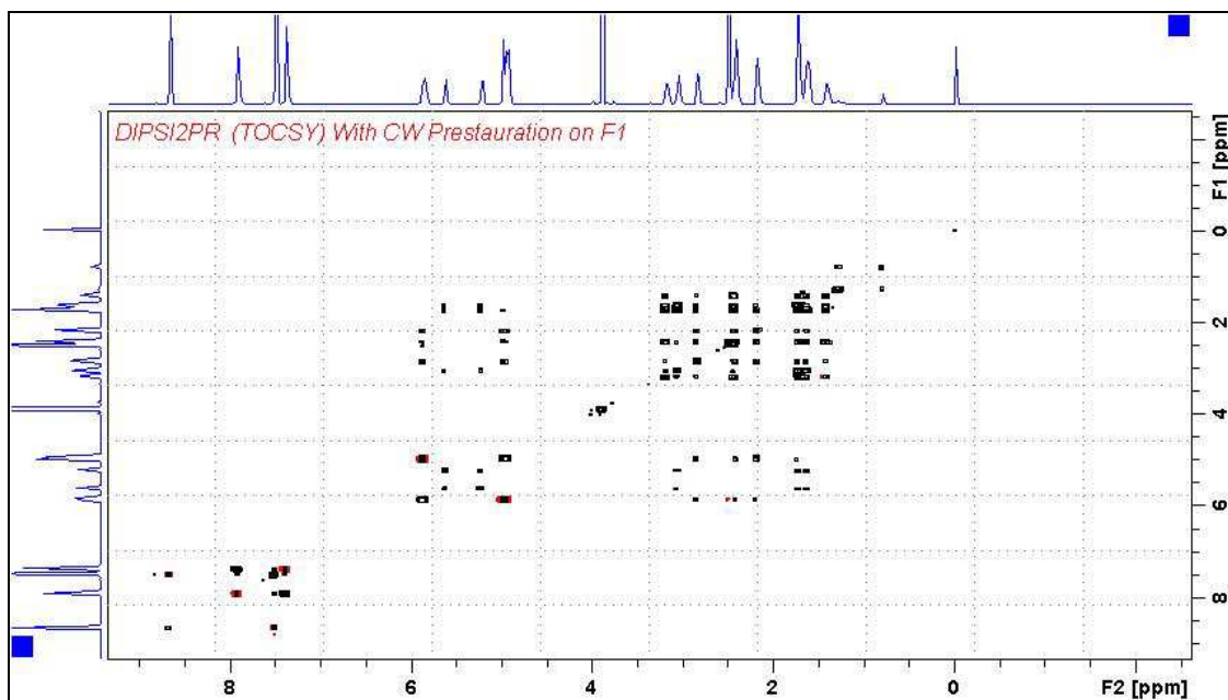
DIPSI2PR spectrum of quinine in D 6 -DMSO with the HOD line at 3.38 ppm suppressed. The spectrum is centered at the O1 frequency of the HOD line.
