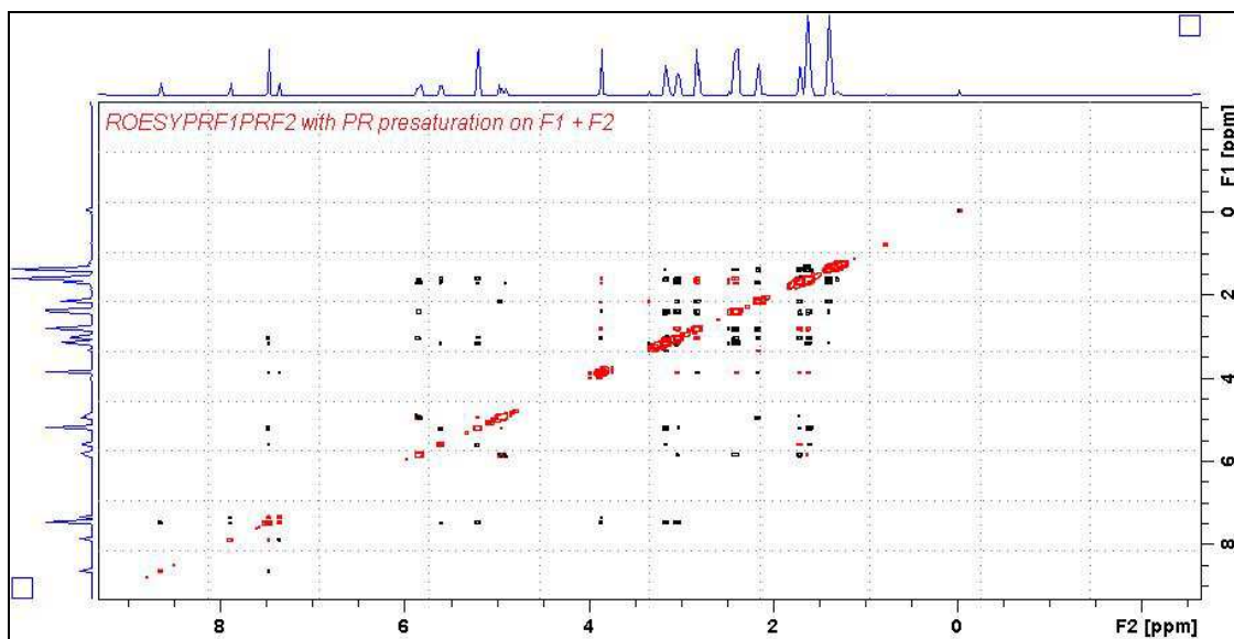
ROESYPRF1PRF2 spectrum of quinine in D 6 -DMSO with the HOD and DMSO lines at 3.38 ppm and 2.5 ppm suppressed. The spectrum is centered at the O1 frequency of the HOD line.
