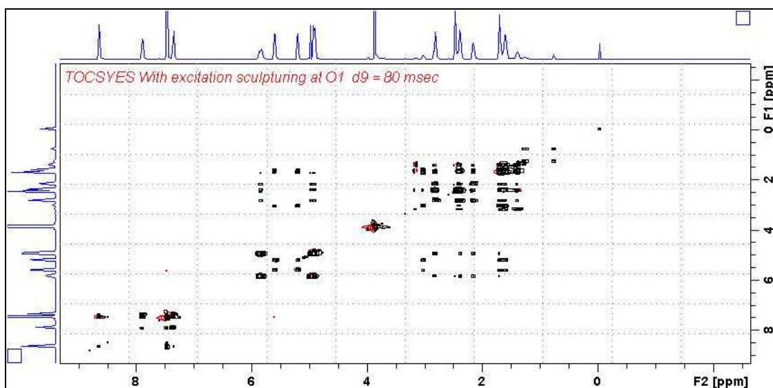
TOCSYES spectrum of quinine in D 6 -DMSO with the HOD line at 3.38 ppm ES suppressed. The spectrum is centered at the O1 frequency of the HOD line.
