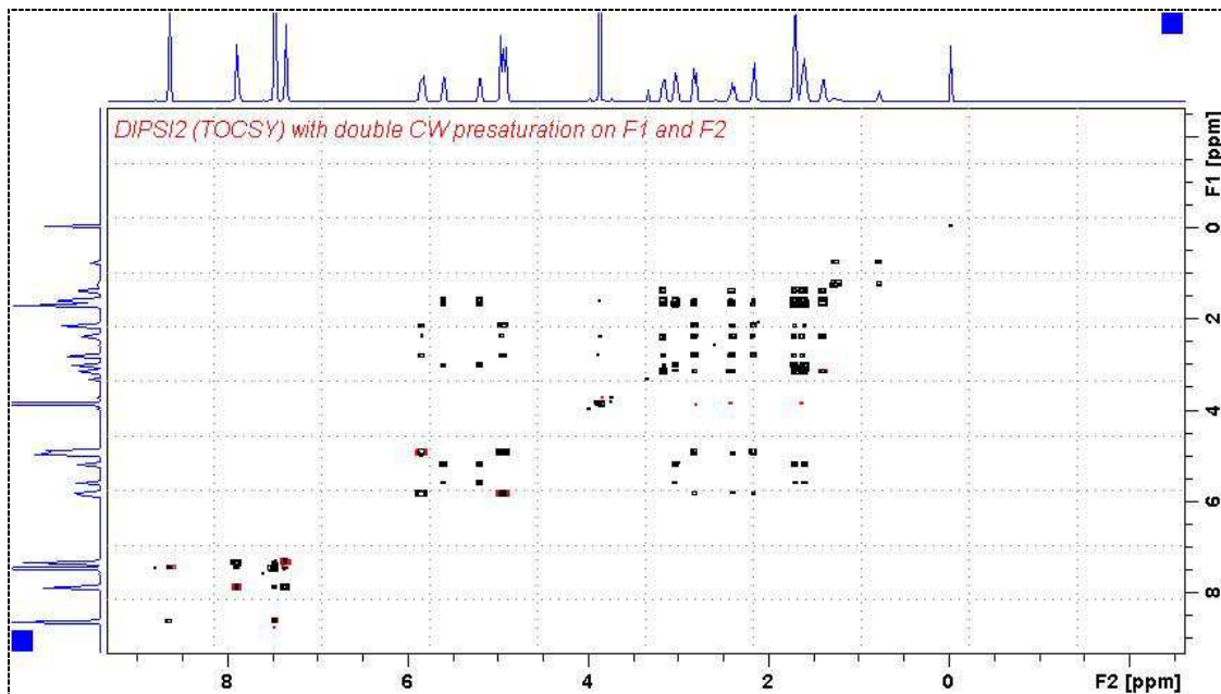
DIPSI2PRF1PRF2 spectrum of quinine in D 6 -DMSO with the HOD and DMSO lines at 3.38 ppm and 2.5 ppm suppressed. The spectrum is centered at the O1 frequency of the HOD line.
