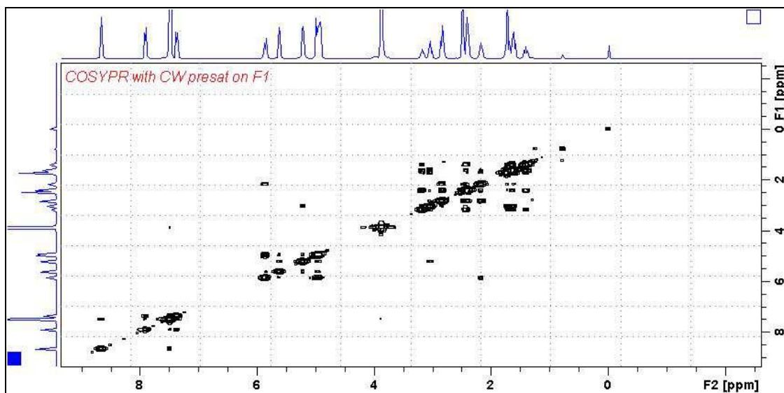
COSYPR spectrum of quinine in D 6 -DMSO with the HOD line at 3.38 ppm suppressed. The spectrum is centered at the O1 frequency of the HOD line.
