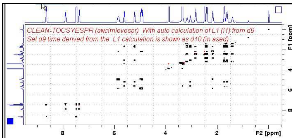
CLEAN-TOCSYESPR spectrum of quinine in D_6 -DMSO with the HOD line at 3.38 ppm ES and PR suppressed. The spectrum is centered at the O1 frequency of the HOD line.
