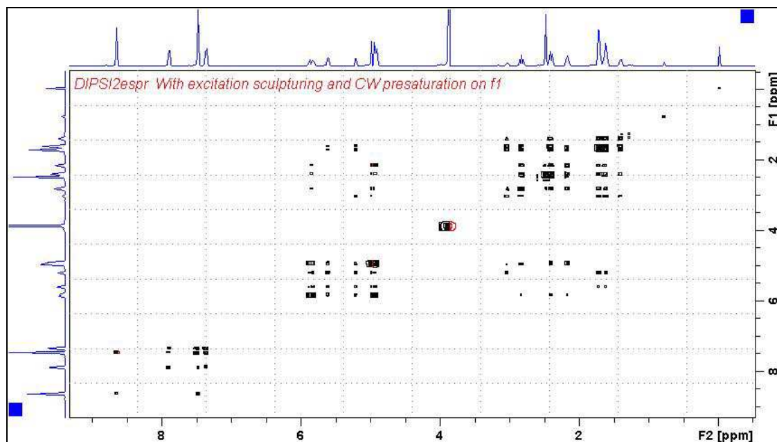
DIPSI2ESPR spectrum of quinine in D 6 -DMSO with the HOD line at 3.38 ppm ES and PR suppressed. The spectrum is centered at the O1 frequency of the HOD line.
