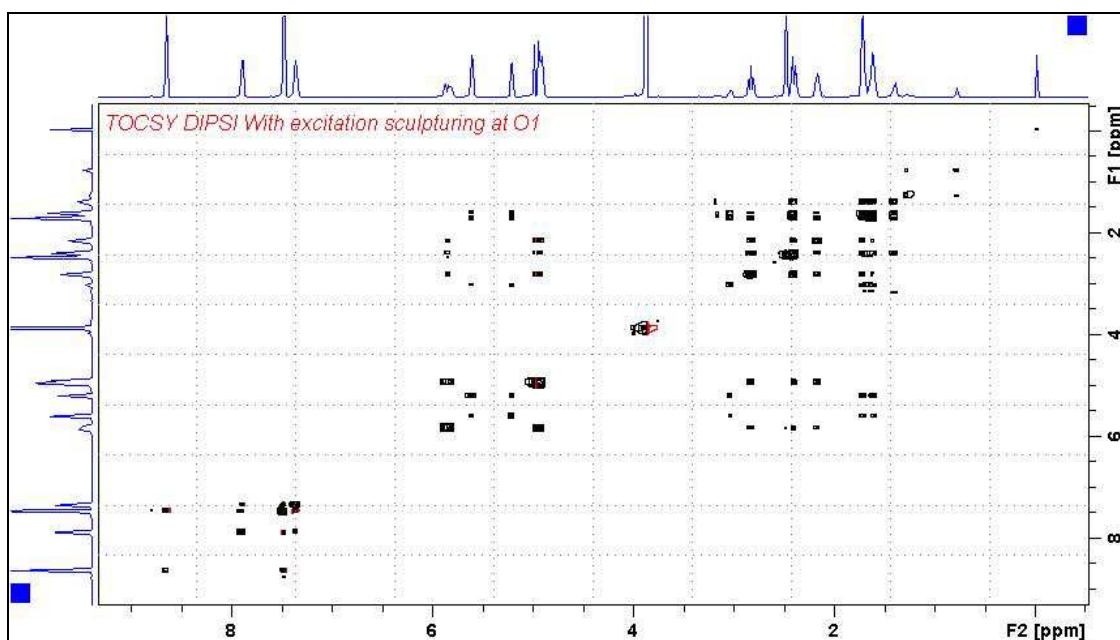
DIPSI2ES spectrum of quinine in D 6 -DMSO with the HOD line at 3.38 ppm ES suppressed. The spectrum is centered at the O1 frequency of the HOD line.
