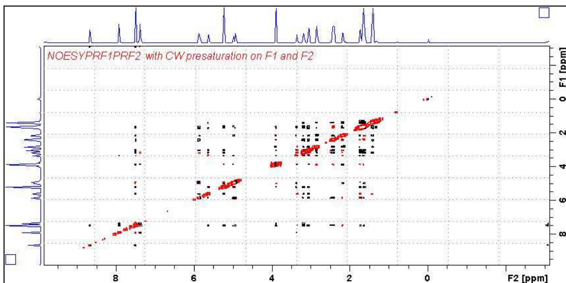
NOESYPRF1PRF2 spectrum of quinine in D 6 -DMSO with the HOD and DMSO lines at 3.38 ppm and 2.5 ppm suppressed. The spectrum is centered at the O1 frequency of the HOD line.
