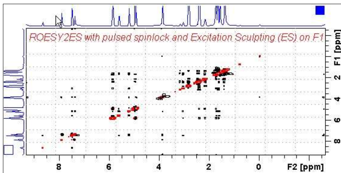
600 MHz ROESY2ES spectrum of quinine in D_6 -DMSO with the HOD line at 3.38 ppm ES suppressed. The spectrum is centered at the O1 frequency of the HOD line.
