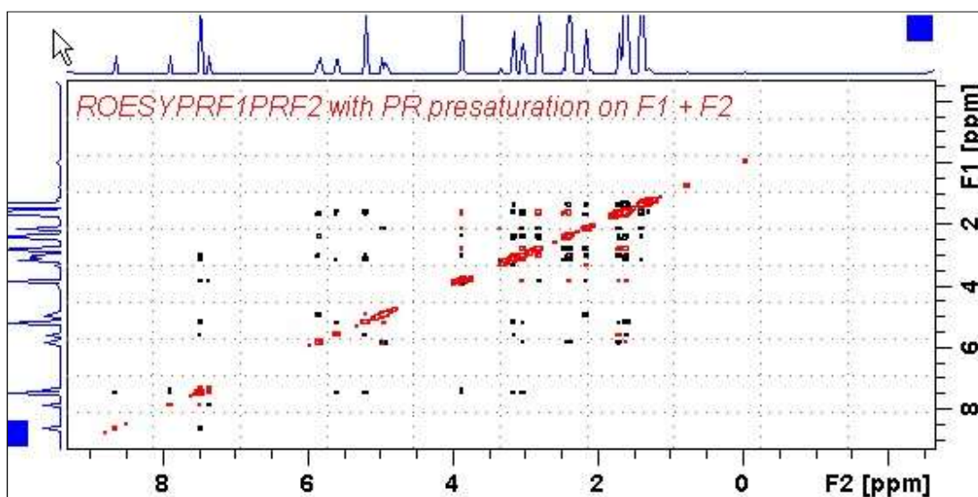
600 MHz ROESYPRF1PRF2 spectrum of quinine in D 6 -DMSO with the HOD and DMSO lines at 3.38 ppm and 2.5 ppm suppressed. The spectrum is centered at the O1 frequency of the HOD line.
