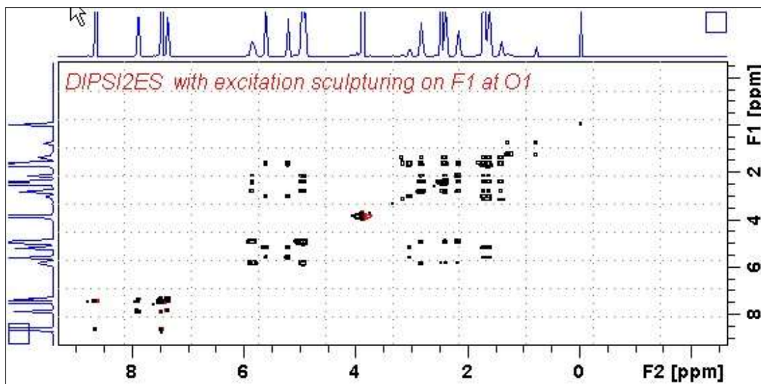
600 MHz DIPSIES spectrum of quinine in D 6 -DMSO with the HOD line at 3.38 ppm ES suppressed. The spectrum is centered at the O1 frequency of the HOD line.
