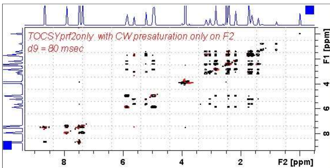
600 MHz TOCSYPRF2ONLY spectrum of quinine in D 6 -DMSO with the HOD line at 3.38 ppm presaturated at O2 on F2.
