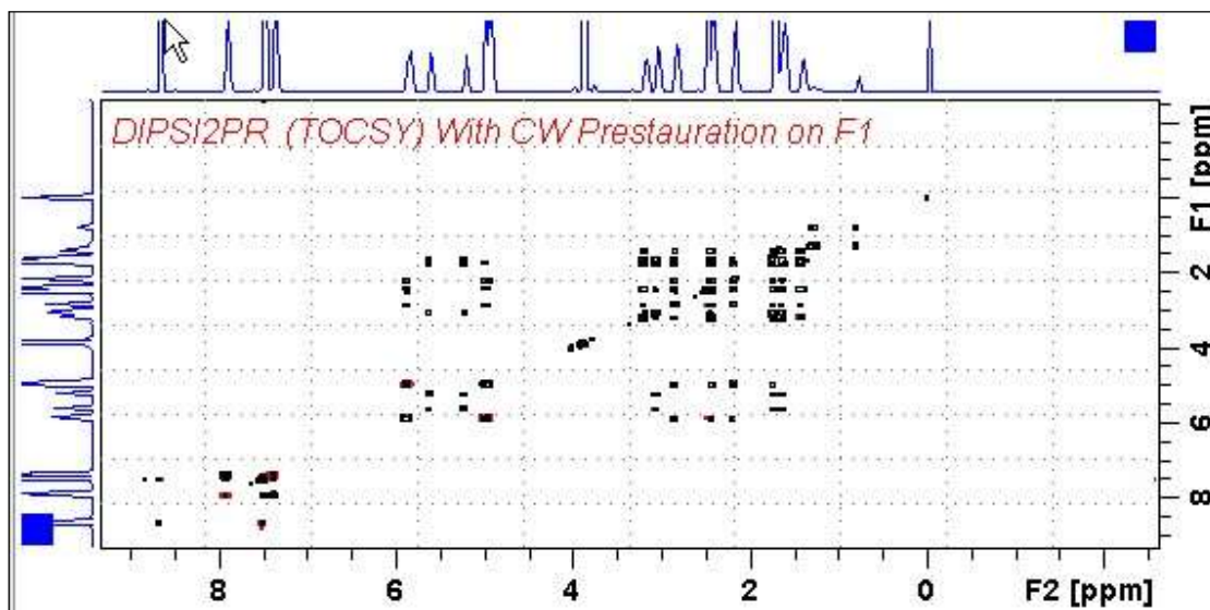
600 MHz DIPS12PR spectrum of quinine in D 6 -DMSO with the HOD line at 3.38 ppm suppressed. The spectrum is centered at the O1 frequency of the HOD line.
