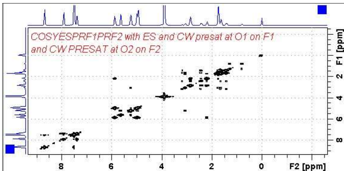
600 MHz COSYESPRF1PRF2 spectrum of quinine in D 6 -DMSO with the HOD line at 3.38 ppm ES and PR suppressed and the DMSO line at 2.5 ppm PR presaturated. The spectrum is centered at the O1 frequency of the HOD line.
