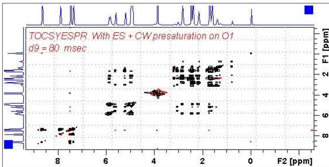
600 MHz TOCSYESPR spectrum of quinine in D_6 -DMSO with the HOD line at 3.38 ppm ES and PR suppressed. The spectrum is centered at the O1 frequency of the HOD line.
