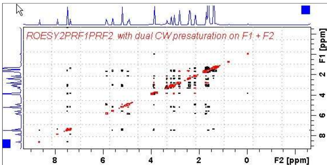
600 MHz ROESY2PRF1PRF2 spectrum of quinine in D 6 -DMSO with the HOD and DMSO lines at 3.38 ppm and 2.5 ppm suppressed. The spectrum is centered at the O1 frequency of the HOD line.
