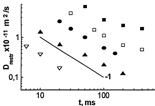
Fig. 2. Plot of \log(D_{restr}) against \log(t_d) for data of Fig. 1.
