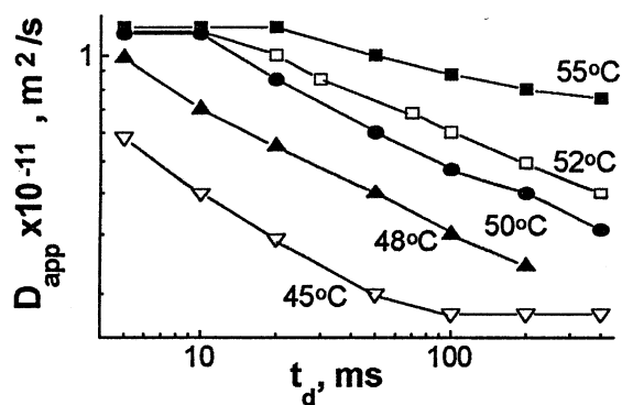
Fig. 1. Plot of the D_{app} against t_d for the mixture with 90% poly(ethylene oxide) crystallized at different temperatures. The temperature of observation is 35°C.
