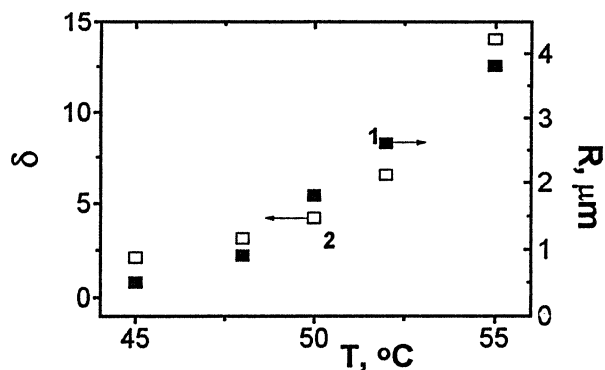
Fig. 3. Plots of size of heterogeneities, R , and parameter \delta against the crystallization temperature for the mixture containing 90% of poly(ethylene oxide).
