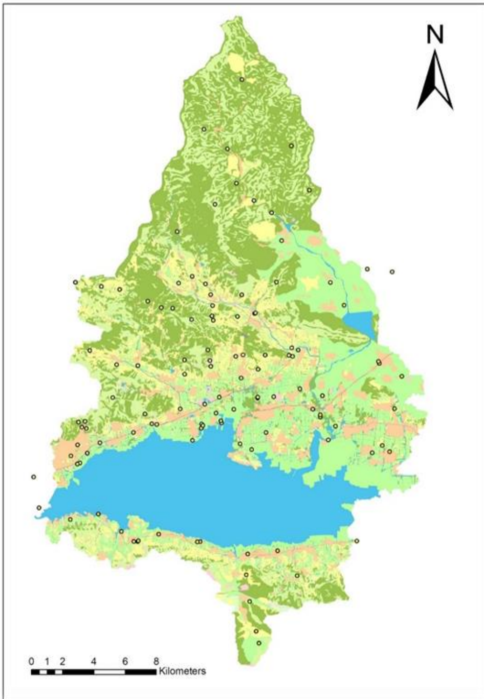
Fig.13 Location of sampling sites around the Yuqiao reservoir
