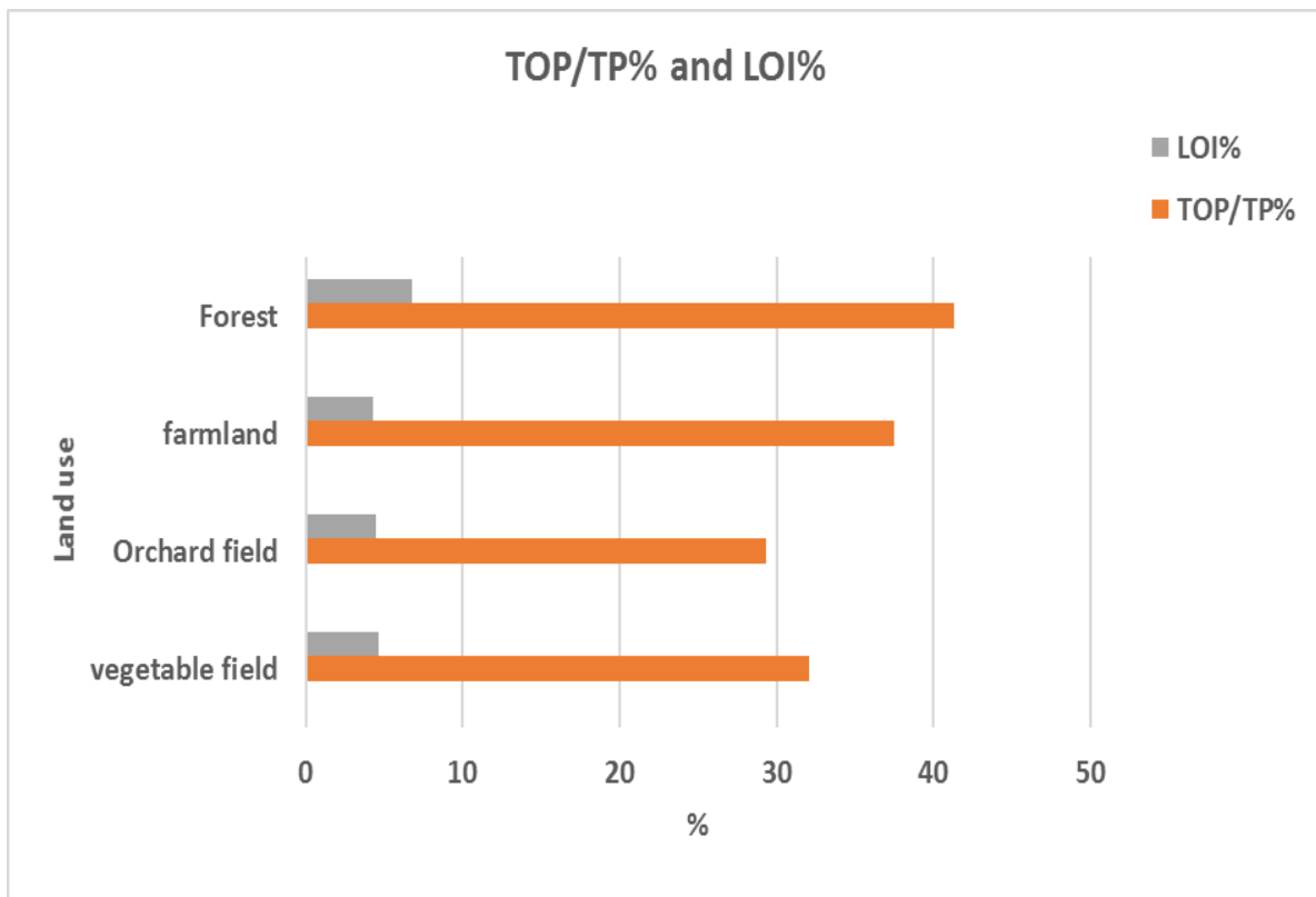
Fig.22 Fraction of Total Organic Phosphorus and LOI%
