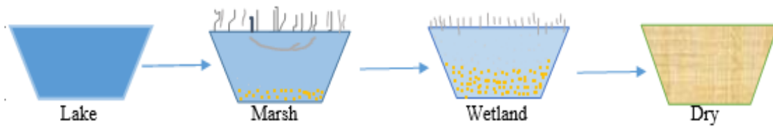
Fig.1 Eutrophication process, showing the progression from aquatic environment to terrestrial environment (Wetzel 1992)
