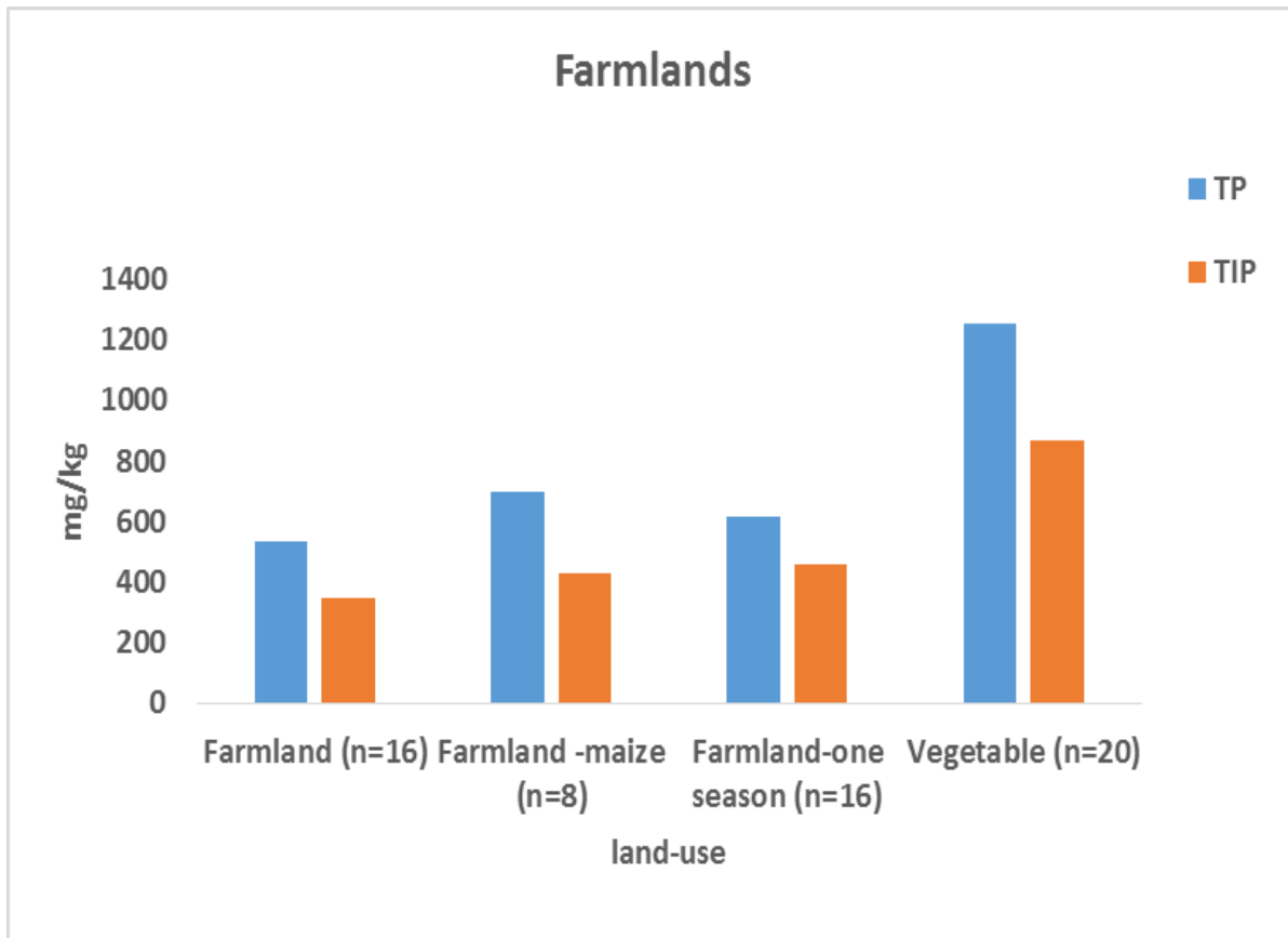
Fig. 20 Total phosphorus (TP) and total inorganic phosphorus (TIP) for different farm practice and Vegetable farm.
