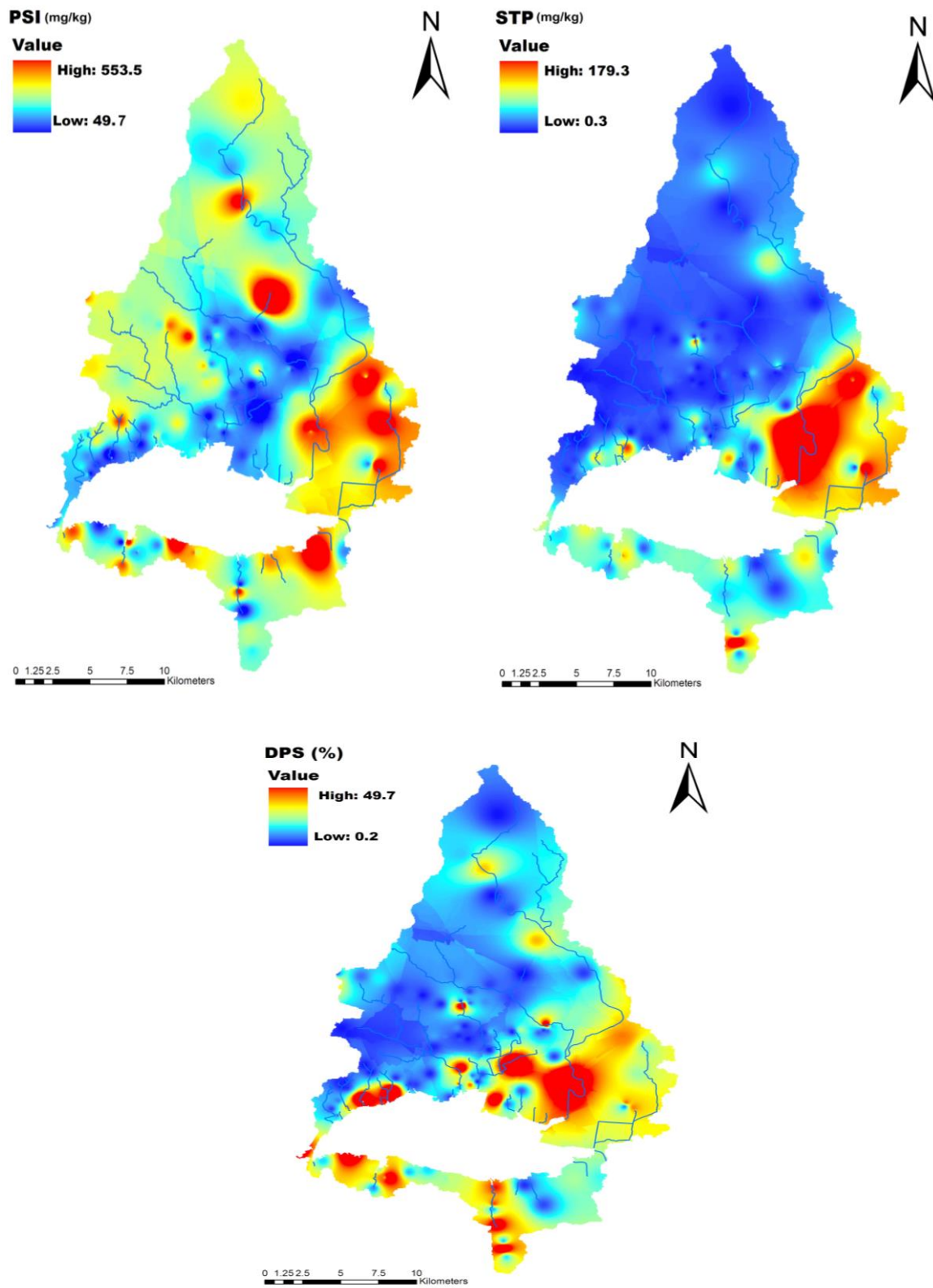
Fig.27 Spatial distribution for Phosphorus Sorption Index (PSI), Bioavailable Phosphorus or Soil Test Phosphorus (BAP or STP) and Degree of Phosphorus Saturation (DPS %)
