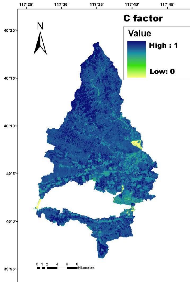
Fig.28 Spatial distribution of C factor
