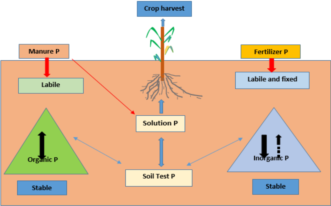
Fig.9 The phosphorus cycle in agricultural soils (USDA, 2003)
