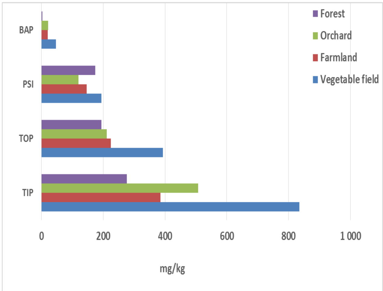
Fig.24 Comparison of Phosphorus pools in top soil (n=126) for different land-use
