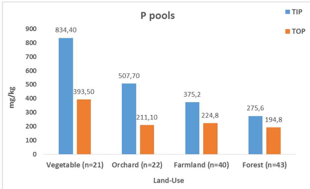
Fig. 17 Phosphorus pools for A-horizons from different land-use
