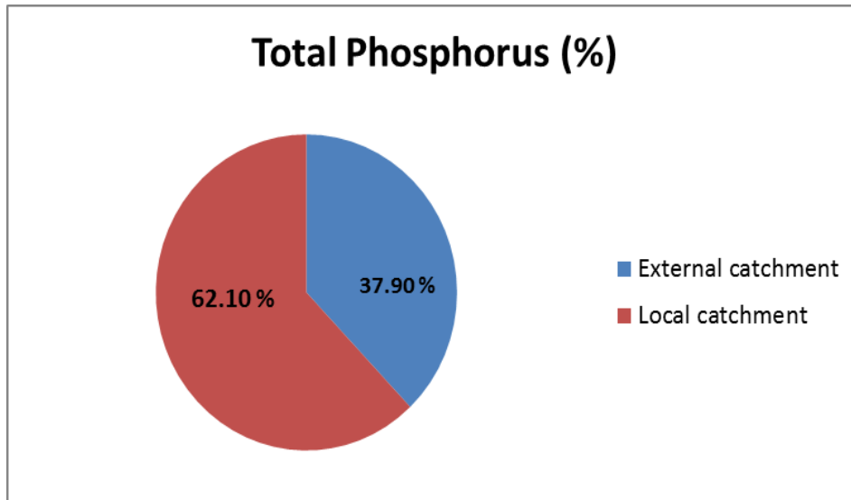
Fig.4 The total phosphorus contribution from local and external catchment (data source: Ji county Environmental Protection Bureau)
