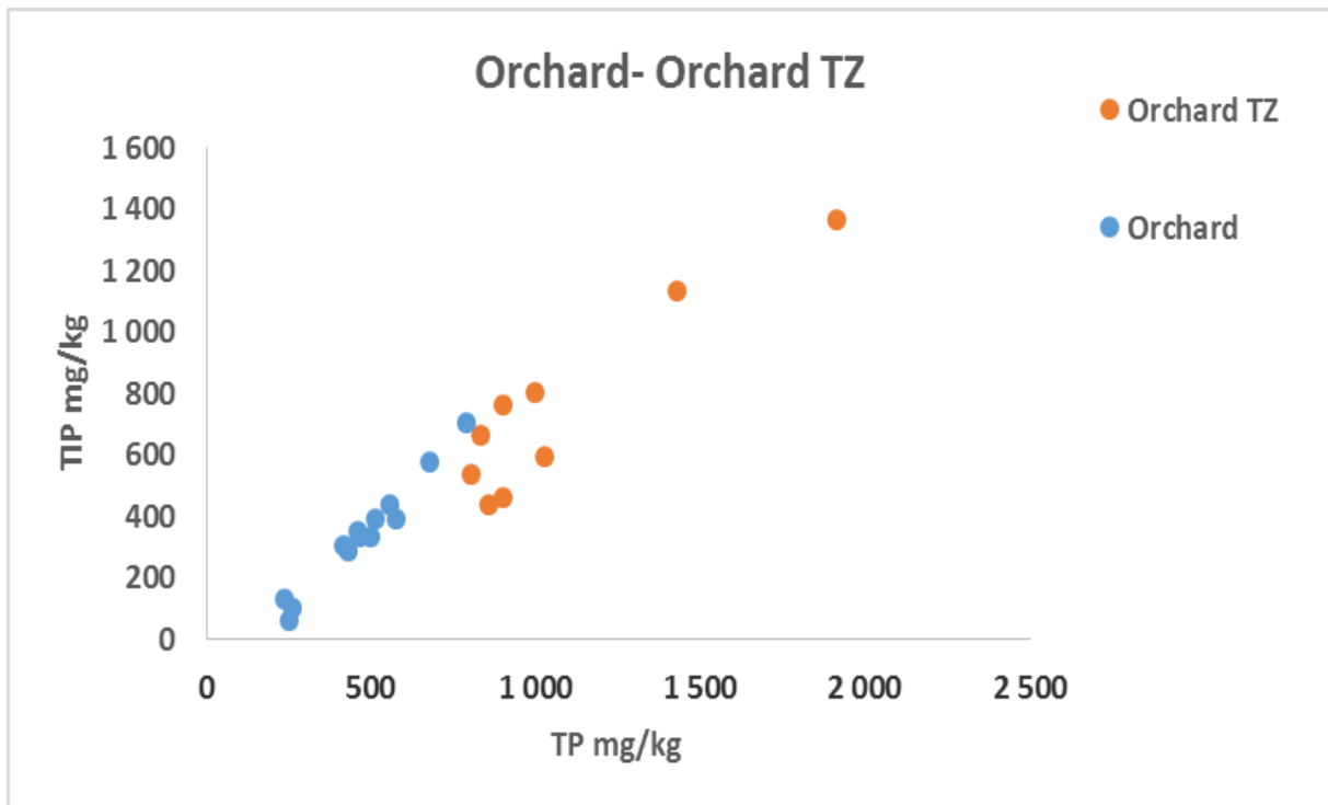
Fig.21 Total phosphorus (TP) and total inorganic phosphorus (TIP) for Orchard- Orchard (tree zone).
