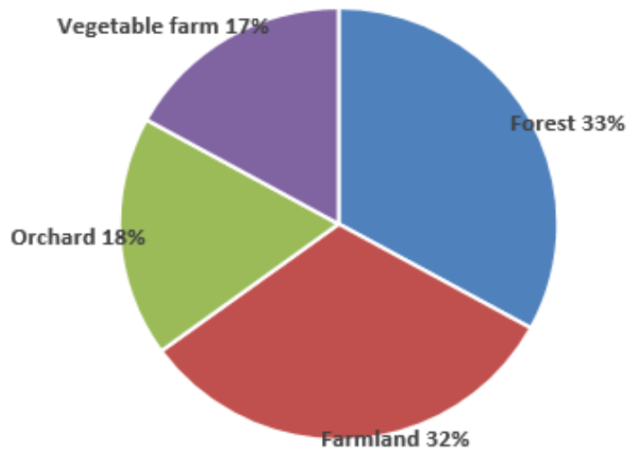
Fig.12 Sampling distribution from different land use.
