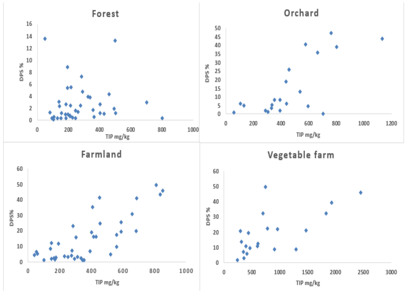
Fig.25 Degree of Phosphorus and TIP for different land use
