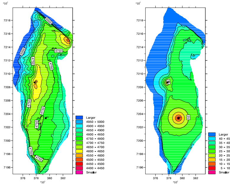
Figure 7: Left panel: predicted depth to eroded surface. Right panel: predicted error to eroded surface.
