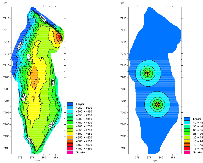
Figure 6: Left panel: predicted depth to eroding surface. Right panel: predicted error to eroding surface.
