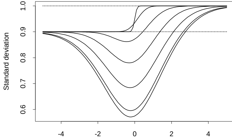
Figure 3: Standard deviations as a function of \mu_2 . The dotted lines are \sigma_1 = \frac{9}{10} and \sigma_2 = 1 . The solid curves are standard deviations of \max(X, Y) for \rho = -1, -9/10, -1/2, 0, 1/2, 9/10 , and 1 . The lowest solid curve is for \rho = -1 .
