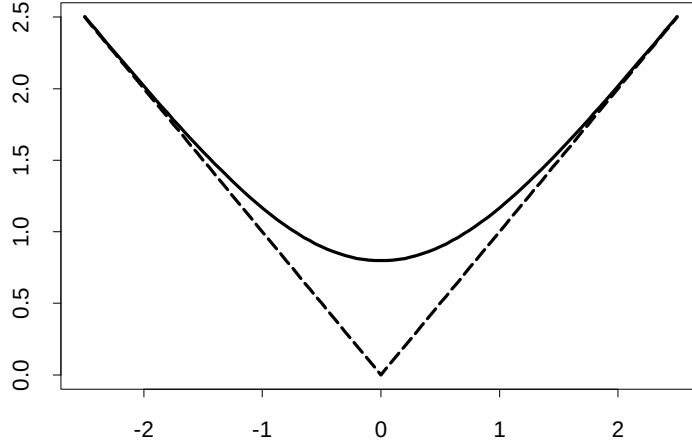
Figure 1: The function A(u) . The dashed lines are |u| .
