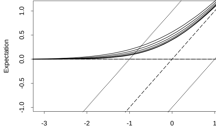
Figure 4: Expectations as a function of \mu_2 . The two dashed lines are \mu_1 and \mu_2 . The solid curves are the expectation of \max(X, Y) for \sigma_1 = 0, 0.2, 0.4, 0.6, 0.8 , and 1 . The deepest curve corresponds to \rho = 1 .
