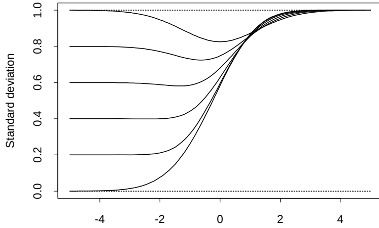
Figure 5: Standard deviations as a function of \mu_2 . The dotted lines are \sigma_1 = 0 and \sigma_2 = 1 . The solid curves are standard deviations of \max(X, Y) for \sigma_1 = 0, 0.2, 0.4, 0.6, 0.8 , and 1 . The lowest curve corresponds to \sigma_1 = 0 .
