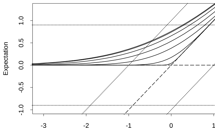
Figure 2: Expectations as a function of \mu_2 . The two dashed lines are \mu_1 and \mu_2 with surrounding dotted lines; \mu_1 \pm \sigma_1 and \mu_2 \pm \sigma_2 . The solid curves are the expectation of \max(X, Y) for \rho = -1, -9/10, -1/2, 0, 1/2, 9/10 , and 1. The solid curve closest to the dashed lines corresponds to \rho = 1 .
