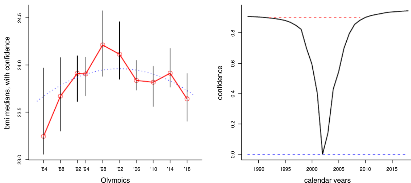
FIGURE 8 Left: Median BMI for men, 10 last Olympics 1984 Sarajevo to 2018 Sochi, with 90% confidence band, and the fitted parabola (19). Right: Focused fusion confidence curve for x^* = -\beta_1 / (2\beta_2) , the maximum point for the parabola in the model for Olympic BMI medians [Color figure can be viewed at wileyonlinelibrary.com ]
