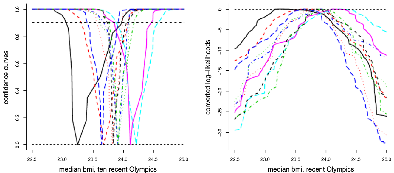
FIGURE 7 Left: Nonparametric confidence curves cc_j(\mu_j) for the medians of the BMI distributions, for the 10 last Olympics 1984 to 2018. Ninety percent confidence intervals are read off from the horizontal dashed line at 0.90. Right: Converted log-likelihood contributions \ell_{\text{conv},j}(\mu_j) for the 10 Olympic medians [Color figure can be viewed at wileyonlinelibrary.com ]
