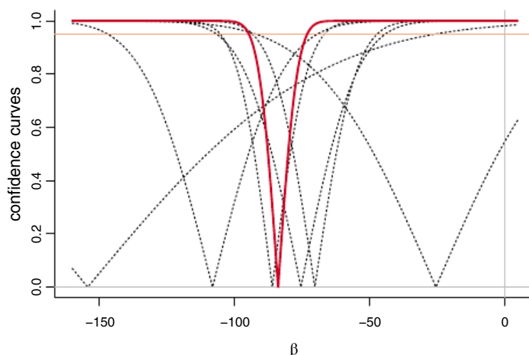
FIGURE 1 Confidence curves for the treatment effect in the six continuous trials (dashed, black). In red, the confidence curve combining all the 11 studies. The horizontal red line marks the 95% confidence level. The median confidence estimate is -83.7 ml, with 95% interval [-94.4, -73.1] [Color figure can be viewed at wileyonlinelibrary.com ]
