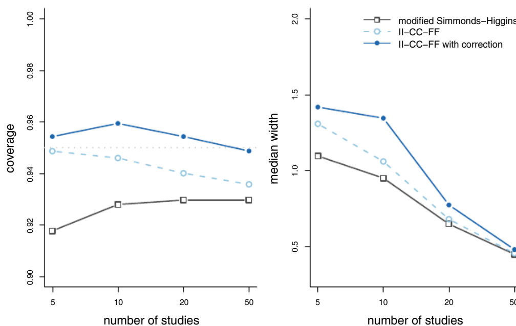
FIGURE 4 Simulation results for random effect meta-analysis of 2 \times 2 tables. The left plot gives the realized coverage rate of 95% confidence intervals, the right plot gives the median width of these intervals [Color figure can be viewed at wileyonlinelibrary.com ]
