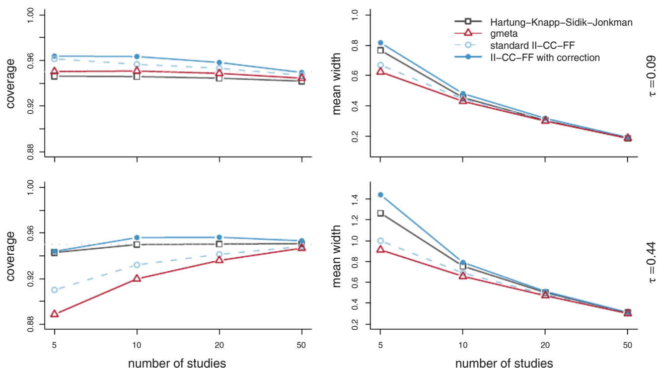
FIGURE 2 Simulation results for the basic random effect model. The left column gives the realized coverage rate of 95% confidence intervals, the right column gives the mean width of these intervals. The results in the top row belong to a scenario with small between-study heterogeneity, while in the bottom row the between-study heterogeneity is large [Color figure can be viewed at wileyonlinelibrary.com ]
