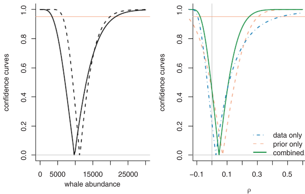
FIGURE 6 Left panel: Confidence curves for \psi_1 and \psi_2 , the abundance of humpback whales in the North Atlantic in 1995 (fully drawn line) and 2001 (dashed line). Right panel: The confidence curve for \rho = (\psi_2 - \psi_1)/(6\psi_1) based on the two surveys (dot-dashed, blue curve); the confidence curve based on prior information alone (dashed, orange curve); and the confidence curve combining the studies and the prior information (full, green curve). See Section 8.2 and Table 2 [Color figure can be viewed at wileyonlinelibrary.com ]
