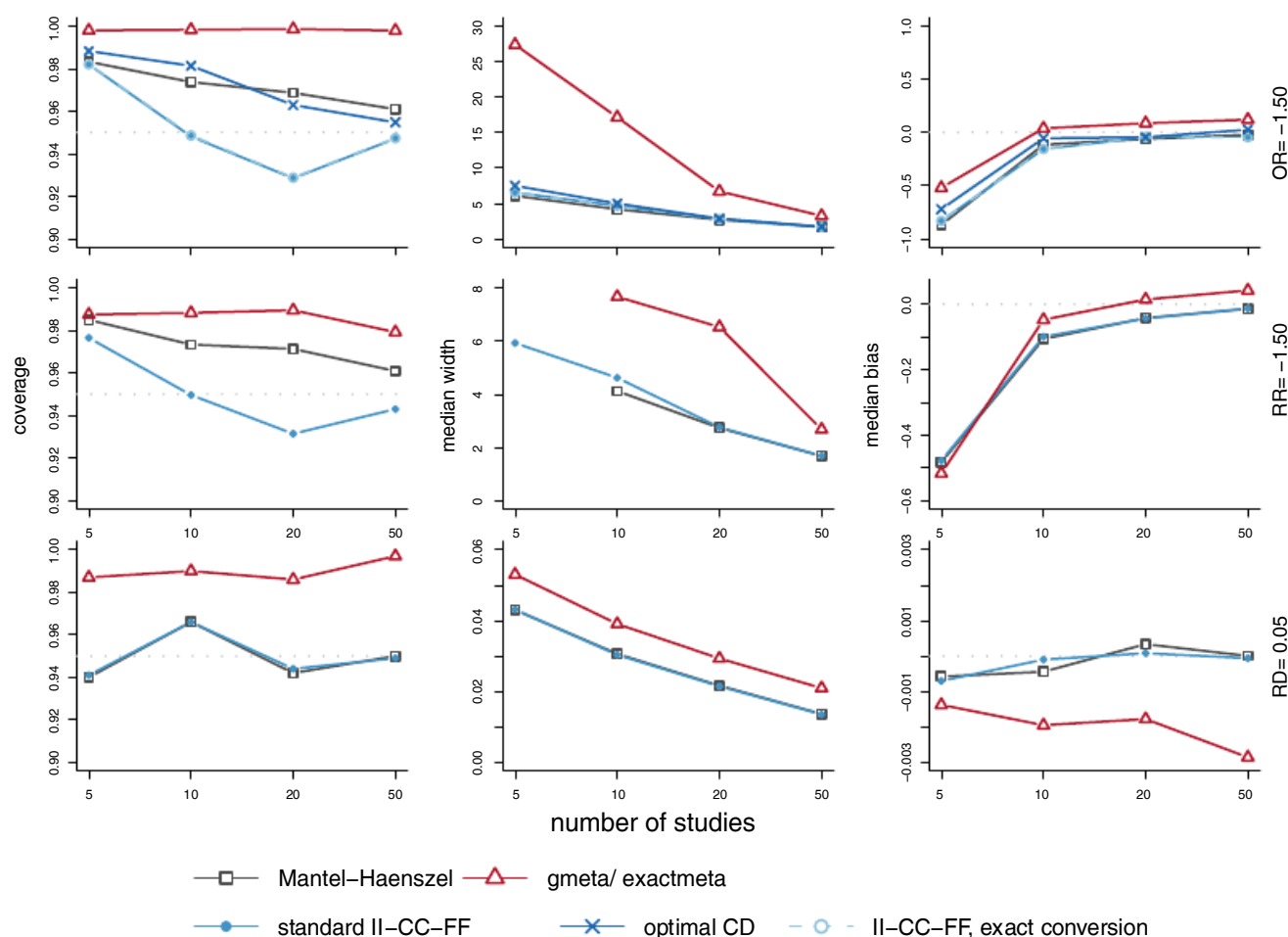
FIGURE 3 Simulation results for fixed-effect meta-analysis of 2 \times 2 tables. The left column gives the realized coverage rate of 95% confidence intervals, the middle column gives the median width of these intervals, and the right column gives the median bias of the point estimate coming from each of the methods. The top row gives the results for the (log) odds ratio, the middle row for the (log) risk ratio, and the bottom row gives the results for the risk difference. When k is small the confidence intervals can sometimes have infinite width (which explains the missing points for the log risk ratio) [Color figure can be viewed at wileyonlinelibrary.com ]
