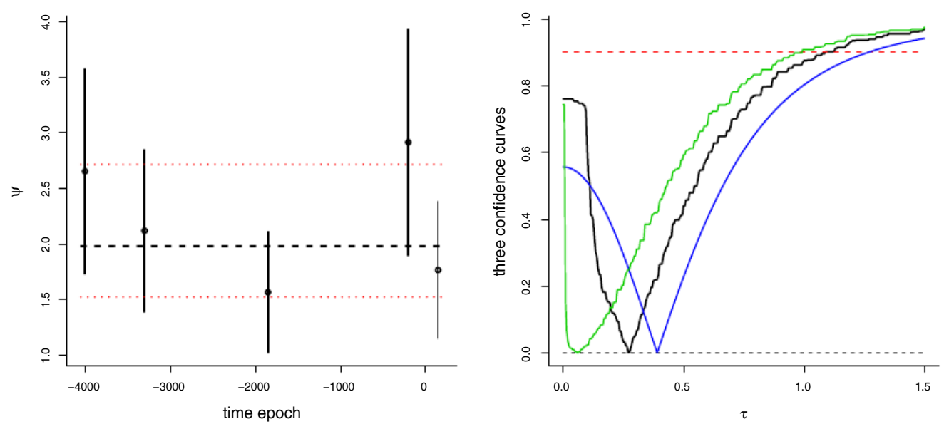
FIGURE 5 Left panel: Point estimates \hat{\psi}_j with 90% confidence intervals, for the skull stretch parameter \psi , across five time epochs (see Table 1). The dashed black line and the red dotted lines indicate the overall point estimate and 90% confidence interval for \psi_0 . Right panel: Three confidence curves for the spread parameter \tau , with median confidence estimates 0.006 (the direct profile method), 0.272 (the corrected profile method), 0.390 (the Q_k(\tau) method) [Color figure can be viewed at wileyonlinelibrary.com ]
