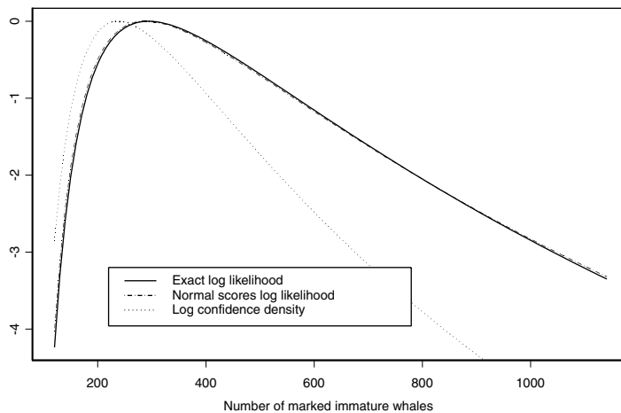
Fig. 4. The exact conditional log-likelihood is shown together with the normal scores log-likelihood and the log-confidence density for the number of marked immature bowhead whales.
