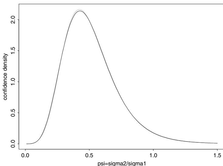
Fig. 3. True confidence density along with abc-estimated version of it (dotted line), for parameter \psi = \sigma_2/\sigma_1 with 5 and 10 degrees of freedom. The parameter estimate in this illustration is \hat{\psi} = 0.50 . The agreement is even better when v_1 and v_2 are closer or when they are larger.
