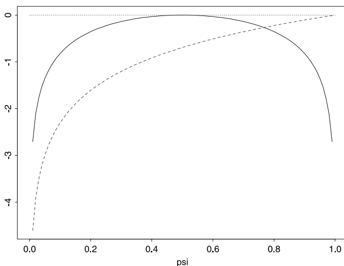
Fig. 1. Three log-likelihoods consistent with a uniform confidence distribution over [0, 1] . "Many likelihoods informed me of this before, which hung so tottering in the balance that I could neither believe nor misdoubt." – Shakespeare .
