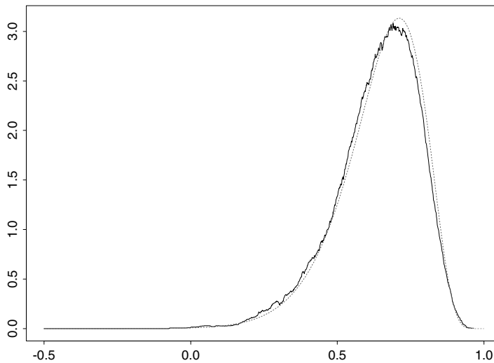
Fig. 2. Approximate confidence density for a binormal correlation coefficient, having observed \hat{\rho} = 0.667 from n = 20 data pairs, via the t -bootstrap method. The confidence density curve is computed via numerical derivation of the C_{tboot}(\rho) curve, using 5000 bootstrap samples. The smoother curve is the simpler version which takes a standard normal for the distribution R .
