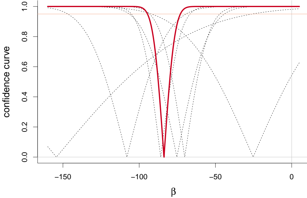
Figure 1.1: Confidence curves for the treatment effect in the six continuous trials (dashed, black). In red, the confidence curve combining all the eleven studies. The horizontal red line marks the 95% confidence level. The median confidence estimate is -83.7 ml, with 95% interval [-94.4, -73.1] .
