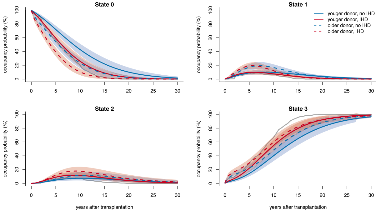
Figure 5. Coloured lines give the fitted occupancy probabilities for the four states (well, mild CAV, severe CAV and death), for patients without (blue) and with (red) IHD and for younger (17 years old, fully drawn) and older (around 40 years old, dashed) patients. The grey line are the non-parametric estimates of the overall state occupancy probabilities. The shaded areas represent the pointwise (approximate) 95% confidence bands (obtained by the delta method). CAV: coronary allograft vasculopathy; IHD: ischaemic heart disease.
