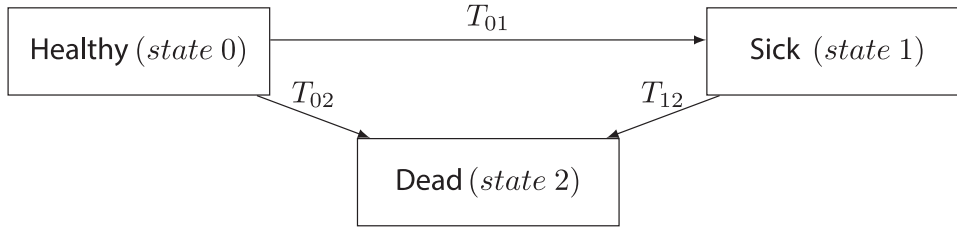
Figure 1. A three-state illness-death model.
