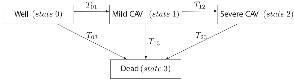
Figure 3. Multi-state graph for the coronary allograft vasculopathy (CAV) dataset – a four-state illness-death model.
