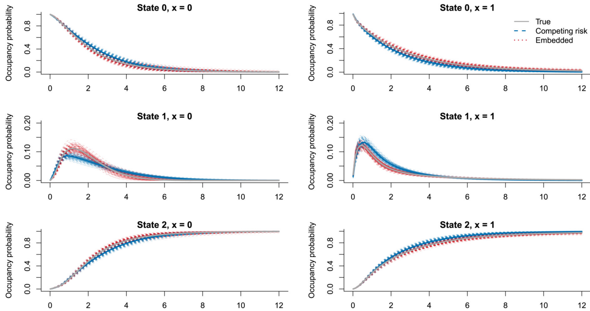
Figure 9. The dashed lines gives the state occupancy probabilities using the estimated parameters for a 100 simulated datasets, for the competing risks approach (blue) and embedded Markov chain approach (red), for x = 0 and x = 1 , when the embedded Markov chain approach is the true simulation model. The true state occupancy probabilities are given by the fully drawn, grey lines.
