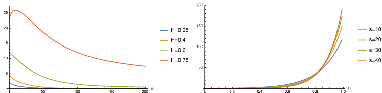
Figure: The covariance function R_H(t, t+s) for \theta = 30 , \sigma = 1 , t = 10 for a non-random I : on the left as a function of s for different values of H ; on the right as a function of H for different values of s .
