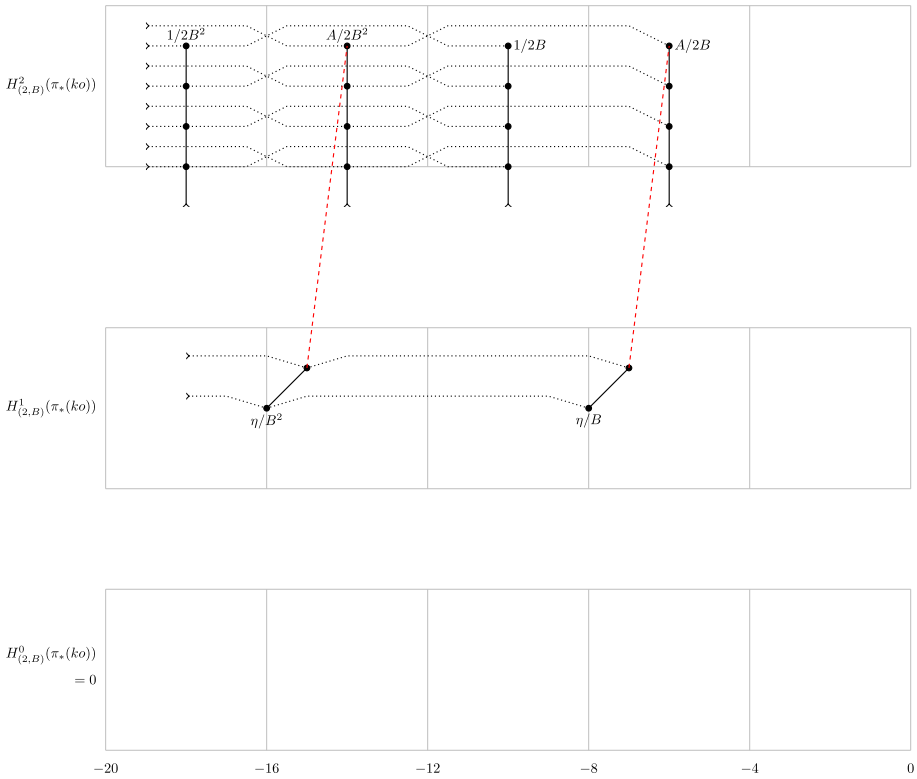
Fig. 2 E_2^{s,t} = H^s_{(2,B)}(\pi_*(ko))_t \implies_s \pi_{t-s}(\Gamma_{(2,B)}ko)
