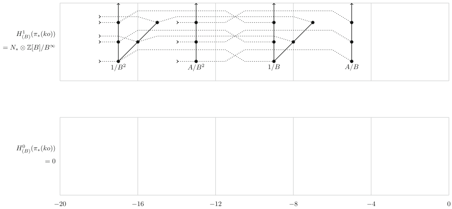
Fig. 1 E_2^{s,t} = H_{(B)}^s(\pi_*(ko))_t \implies_s \pi_{t-s}(\Gamma_B ko)
