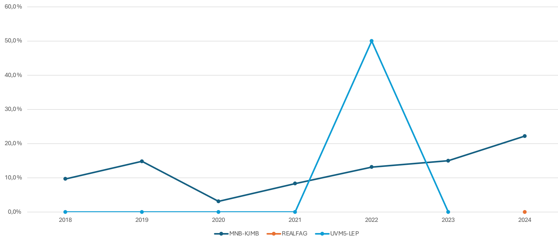
Strykprosent studieprogram
