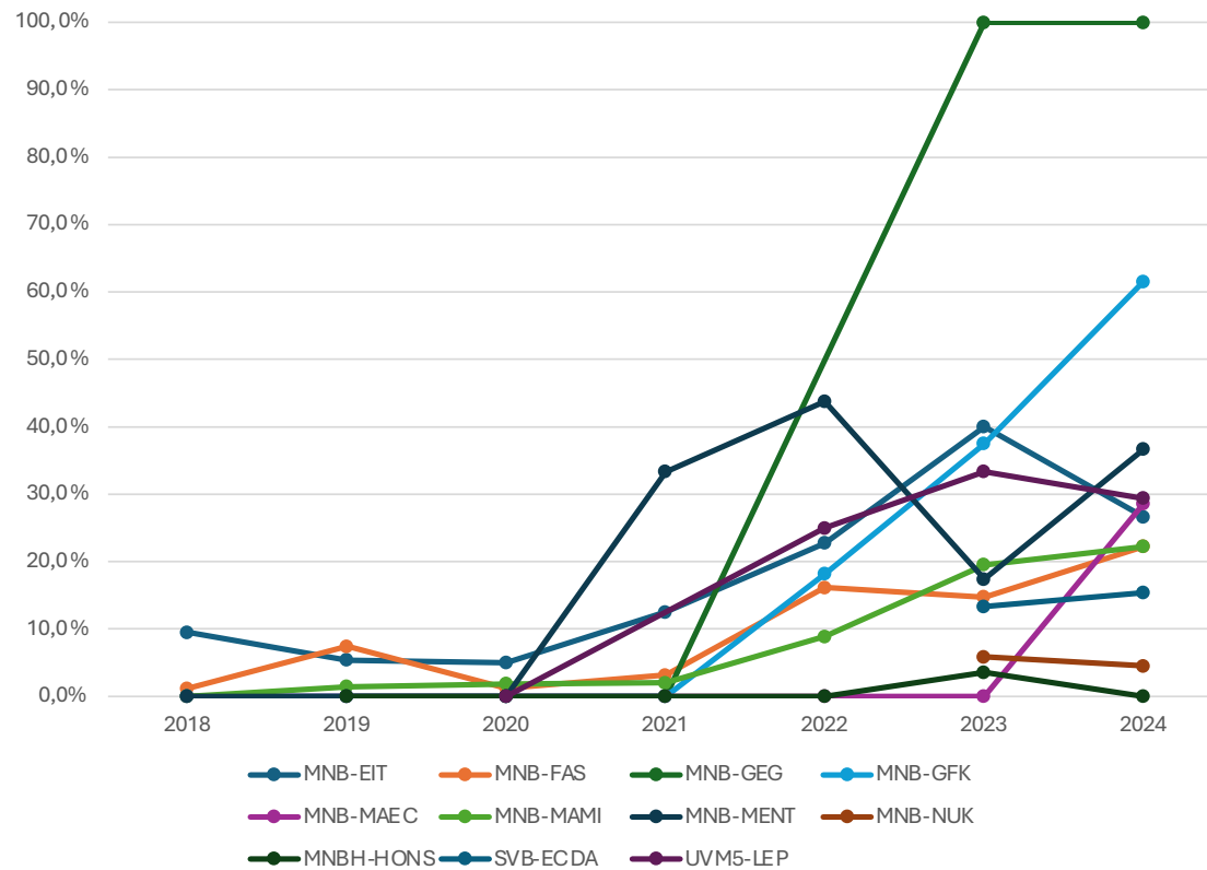
Strykprosent bachelorprogram
