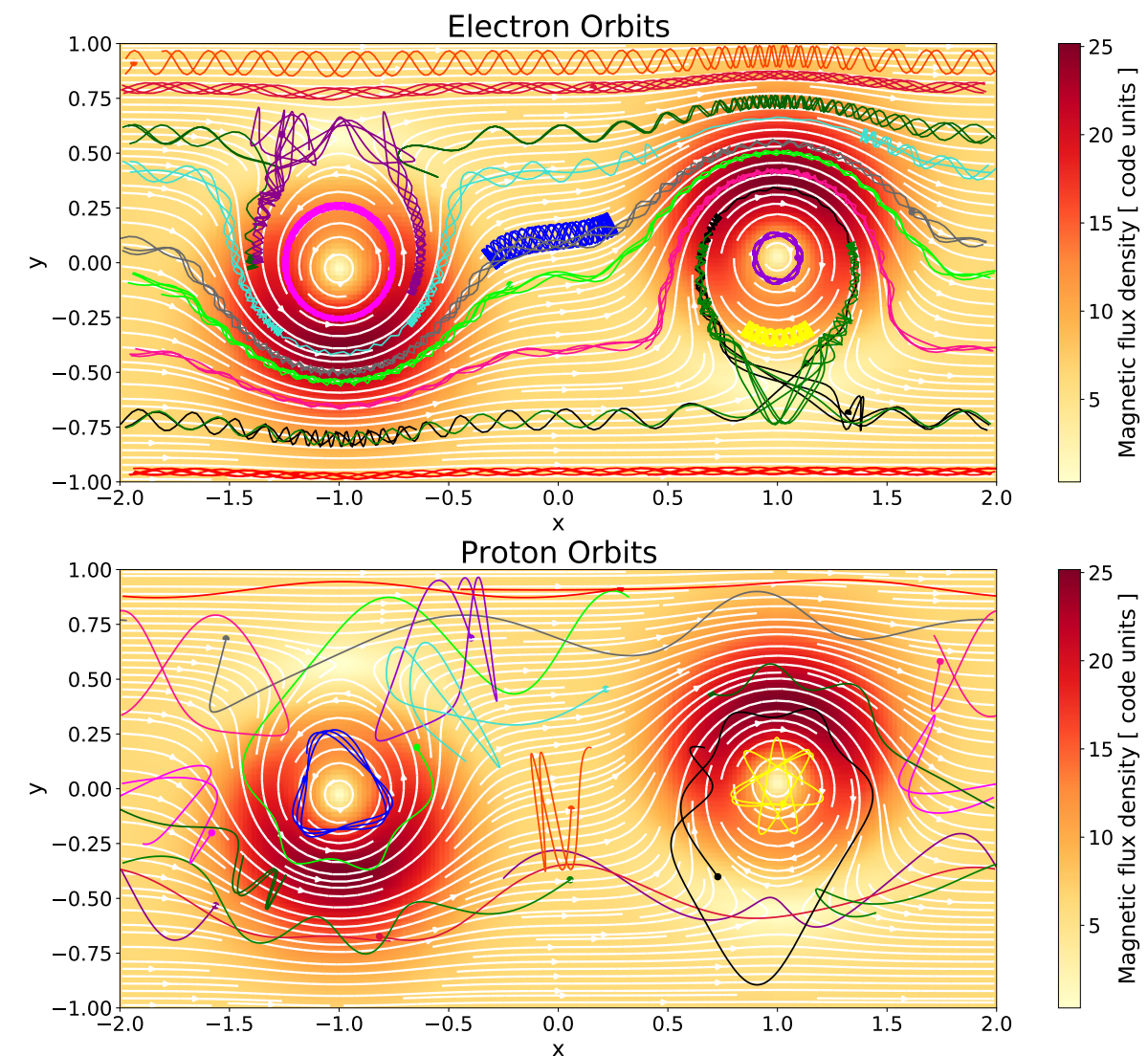
Figure: Example of a simple run with the newly developed particle in cell code. Magnetic field direction is indicated with white stream lines, while particle orbits are shown in different colors.
