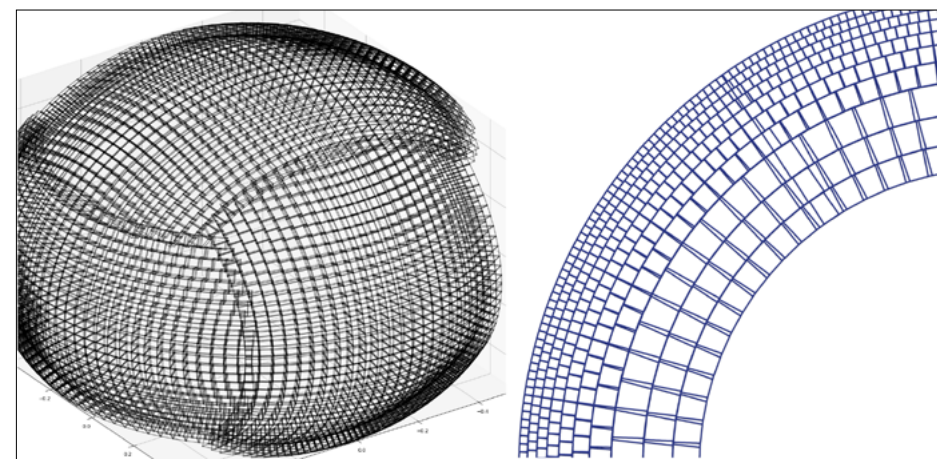
Figure 1. Left: One layer of the ‘volleyball’ mesh. The back side is removed for clarity. Right: Radial cut of the volleyball layers. Adapted from Popovas et al., 2022
